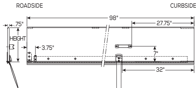
FOR RECESSED 1" WOOD ROLL-UP DOOR
